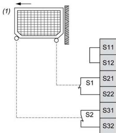
(1): Protective guard
