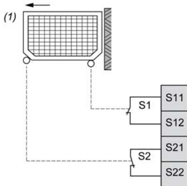
(1): Protective guard
